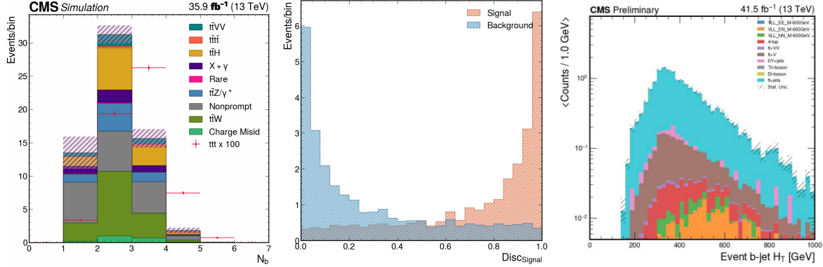
Figure 10: Triple-top analysis: B-jet multiplicity for the signal and background for the triple-top analysis(left), the output of a multivariate discriminant used for signal and background discrimination (middle); VLL analysis: sum of the p_T of the b-tagged jets for the different signal and background contributions (right). [Teague & Pinna; Koraka]
