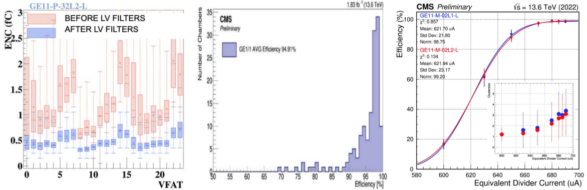
Figure 18: Reduction of noise with low voltage filters installed in different VFATs (left), Efficiency measured in GE/1 detectors during run-3 (center), efficiency as a function of equivalent divider current (as a measure of applied voltage) for GE 1/1 chambers (right).
