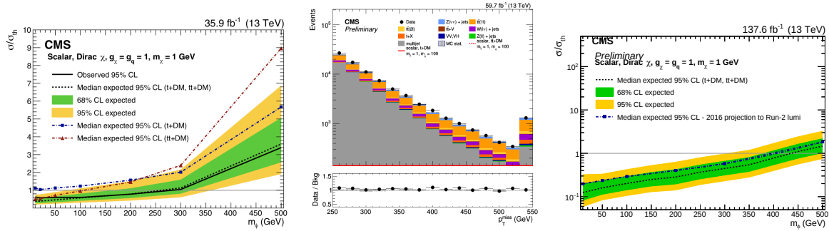
Figure 8: Expected and observed 95% CL upper limits for t\bar{t} + \text{DM} and t + \text{DM} together with their combination (left) for the 2016 analysis [Pinna]. The missing transverse momentum distribution for the data and background for the QCD control region for the 2018 dataset (middle). The expected sensitivity of the full Run 2 analysis compared with the extrapolation of the previous result (using 2016 dataset) to full Run 2 luminosity (right). [Pinna & Shang]
