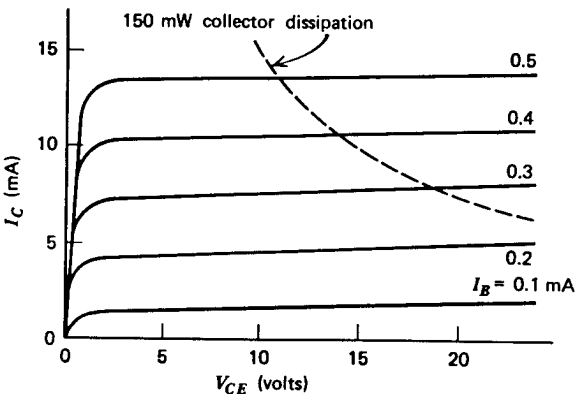
Fig. 8.3 Typical bipolar transistor collector characteristics.
